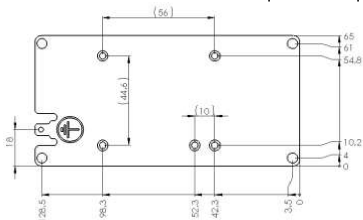
Figure 1.5 Installation plate and dimensions
